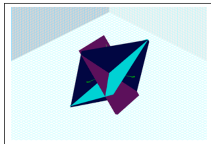
Figure 7: Three planes intersecting in a point
