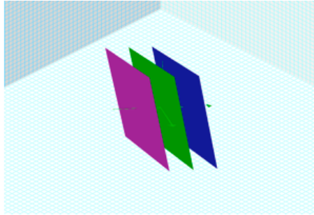
Figure 3: Three parallel planes
