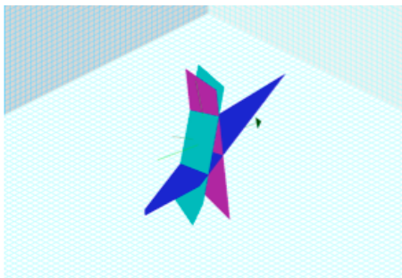
Figure 5: Three planes intersecting pairwise in three parallel lines
