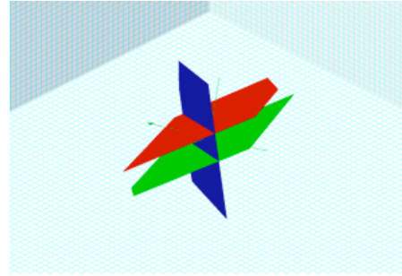
Figure 4: Three planes, two of which are parallel
