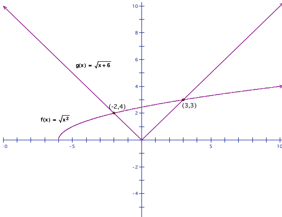
Figure 2: f(x) = \sqrt{x^2} and g(x) = \sqrt{x+6} intersect at x = -2, 3 .
