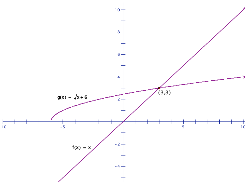
Figure 3: f(x) = x and g(x) = \sqrt{x+6} intersect at x = 3 .
