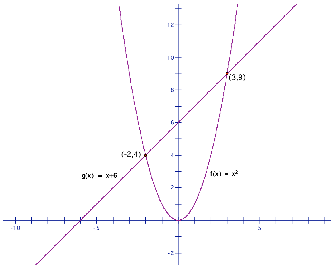
Figure 1: f(x) = x^2 and g(x) = x + 6 intersect at x = -2, 3 .
